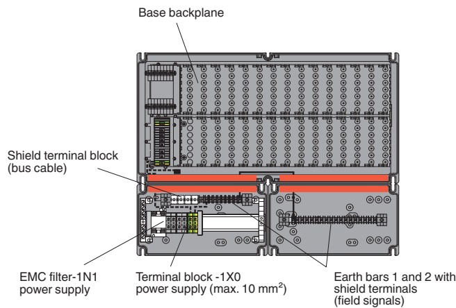
Drawn without cover and cable glands!
