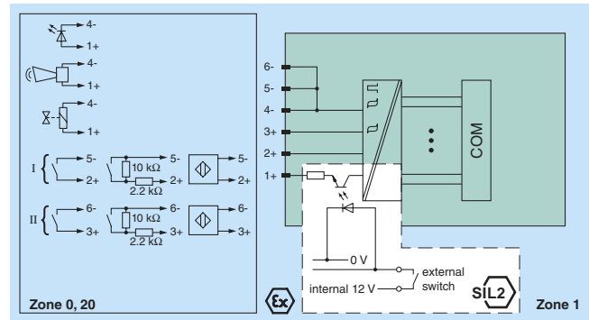
Figure 9 Example: Solenoid driver with valve position feedback
