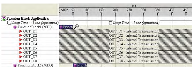
Figure 3 Timing for data acquisition from module to gateway using MFB (host independent)
