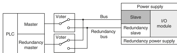
Figure 3 Principle of extended line redundancy: DCS with redundant master master communicating with redundant slaves via two voters or four repeaters
