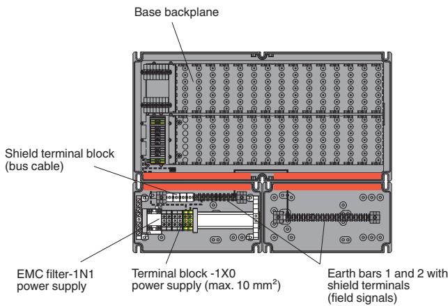
Figure 4 Example backplane
