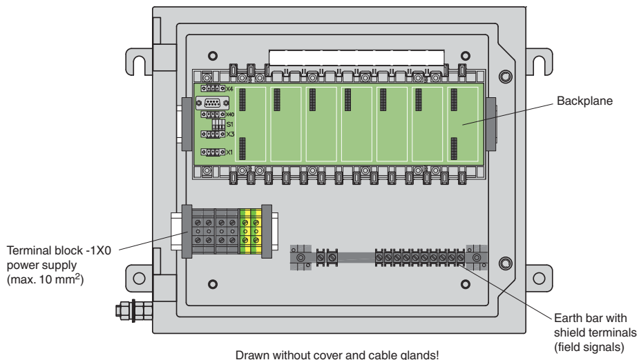
Drawn without cover and cable glands!
