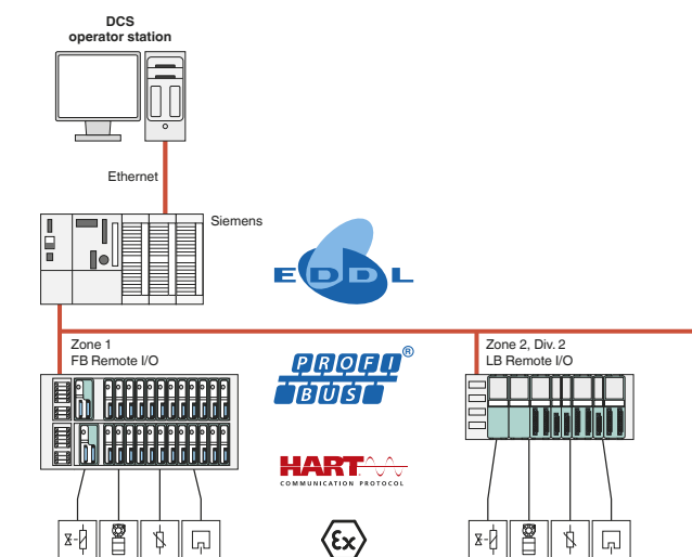
Figure 16 HART through Siemens EDDL technology (S7/400)
