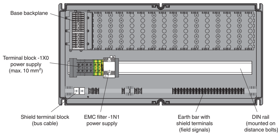
Drawn without cover and cable glands!
