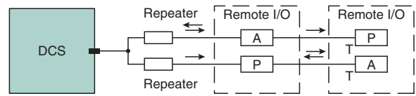
Figure 5 Line redundancy without voter
