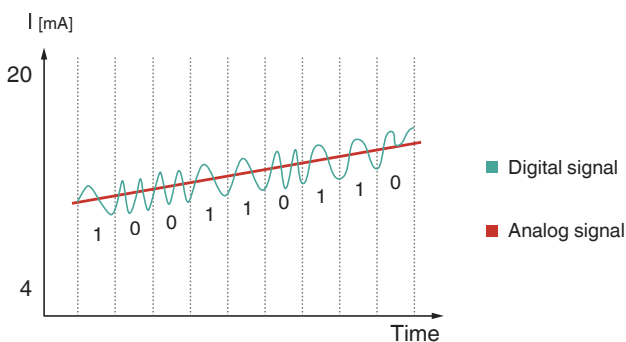
Figure 12 HART modulation of a 20 mA Signal
