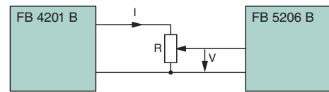
Figure 17 Example Joystick Device Combination for Zone 1
