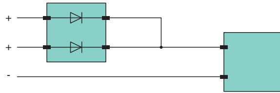
Figure 2 Example diodes allowing redundant power feed
