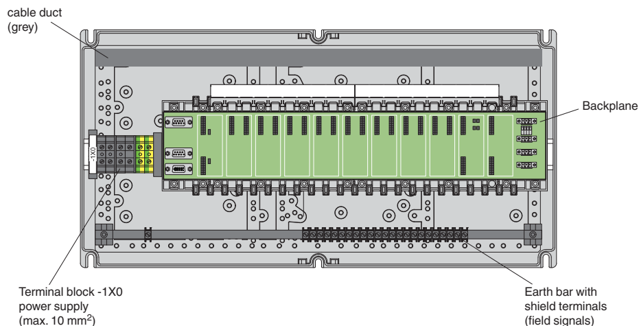
Drawn without cover and cable glands!
