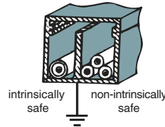
Figure 32 Examples of cable installation
